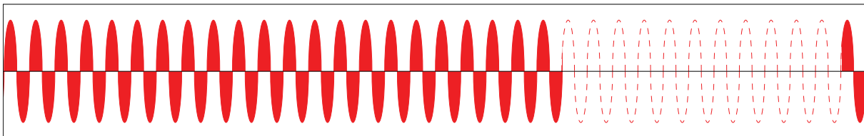
Output with burst firing mode @ 66% control level:
