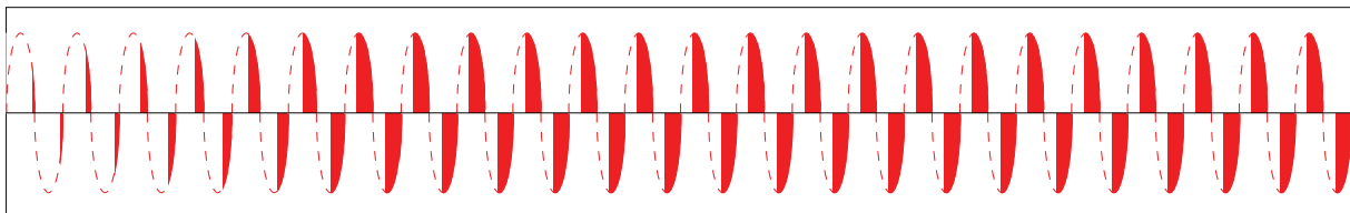
Soft start with phase angle
