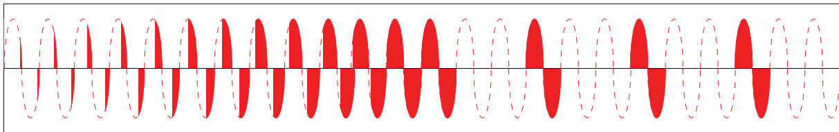
Soft start with ON/OFF, burst, distributed full cycle and advanced full cycle
