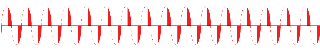
Output with phase angle firing mode @ 33% control level:
